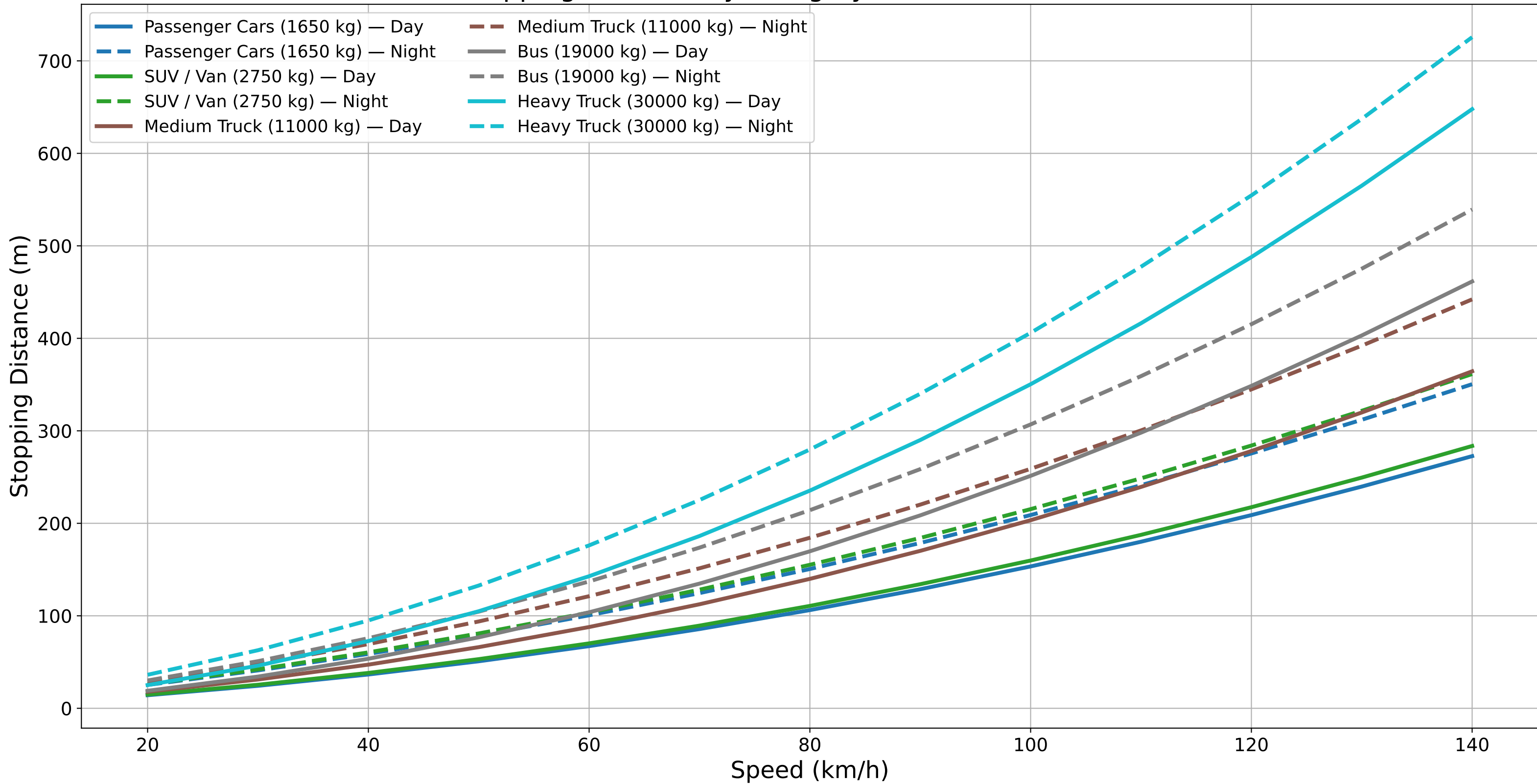
Stopping Distance by Category Under Wet Conditions
