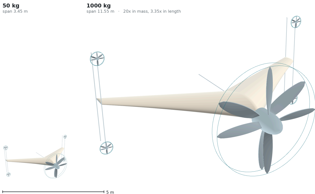
Figure 11. The two reference designs at a common scale: 50 kg and 1000 kg, twenty times apart in mass and 3.35 times in span. Disc loading, energy-buffer mass fraction and tip-frame drag fraction are preserved across that range; transition time is not, and neither is the ratio of propeller diameter to span, which rises from 0.35 to 0.47 because holding the disc loading makes the propeller grow faster than the airframe.
