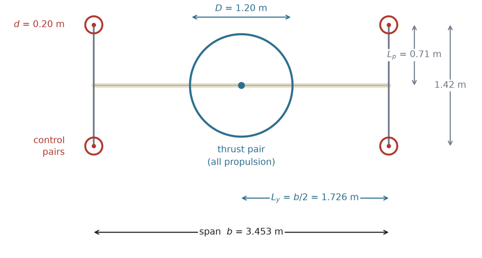
Propeller placement and moment arms — front view
