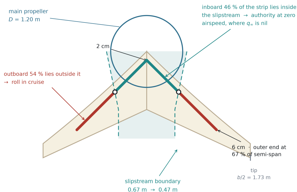
Roll strip and the main-propeller slipstream — view from below
