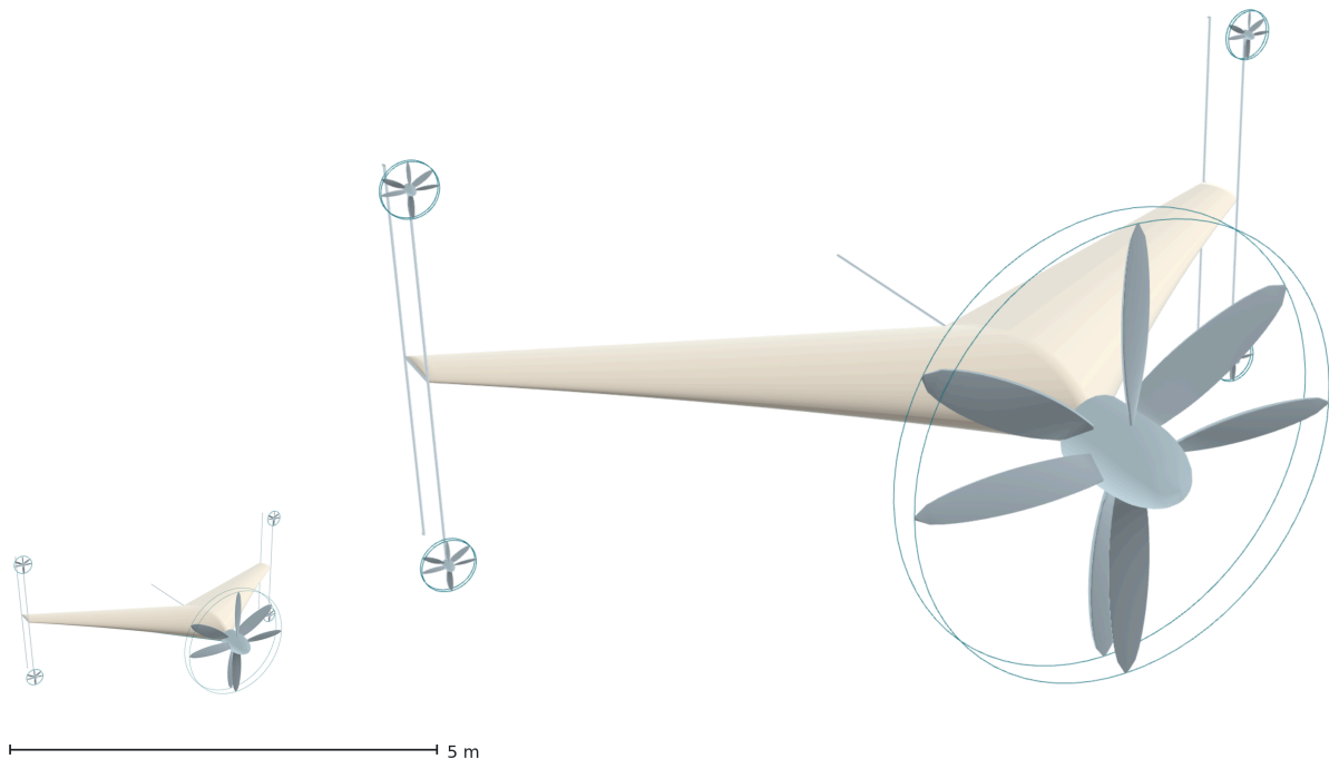
Figure 10. The two reference designs at a common scale: 50 kg and 1000 kg, twenty times apart in mass and 3.35 times in span. Disc loading, energy-buffer mass fraction and tip-frame drag fraction are preserved across that range; transition time is not, and neither is the ratio of propeller diameter to span, which rises from 0.35 to 0.47 because holding the disc loading makes the propeller grow faster than the airframe.
