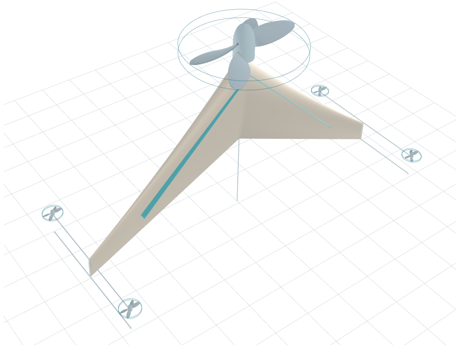
Fig. 1 The 50 kg reference design standing on its tail: nose pair uppermost, tip frames and keel on the ground, strip on the lower surface; blades schematic
