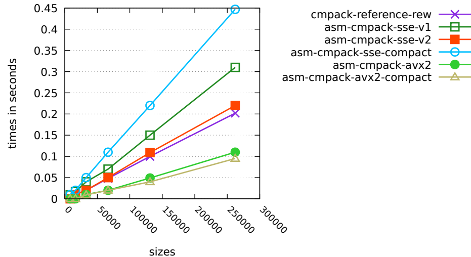
Best methods below average 0.47
