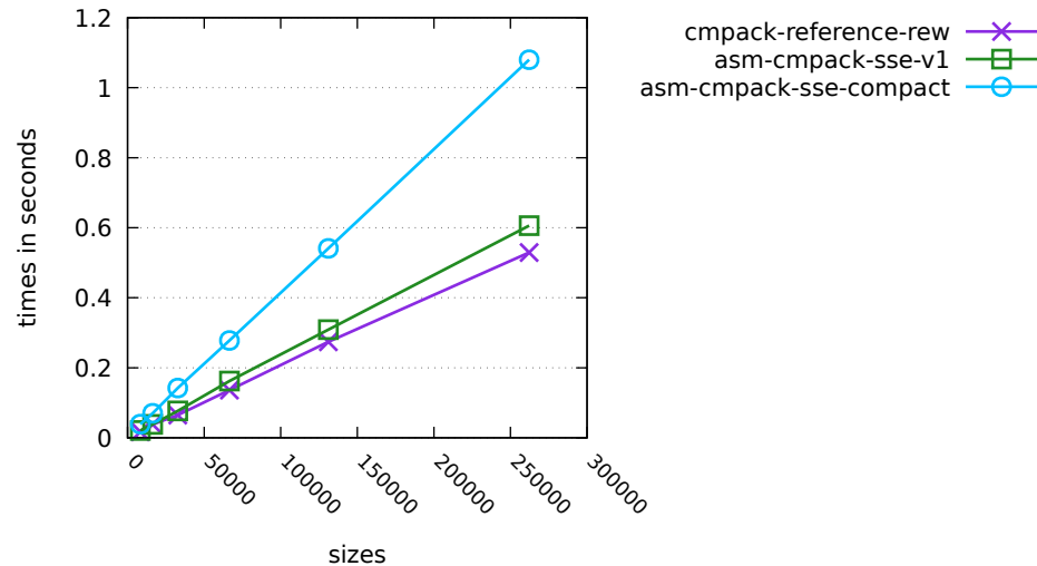
Best methods below average 1.34
