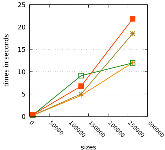
Best methods below average 32.32
