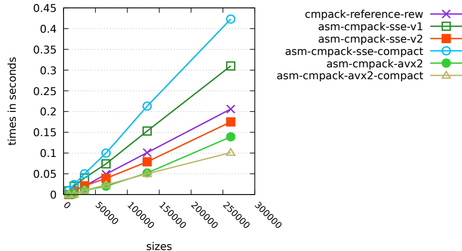
Best methods below average 0.45
