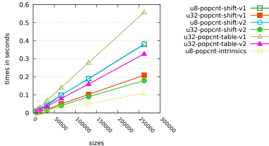
Best methods below average 2.07
