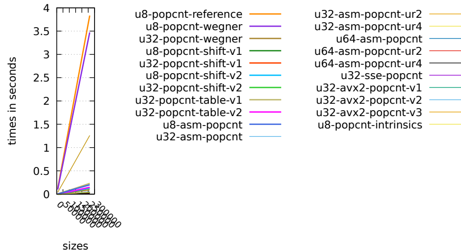
Performance of all methods
