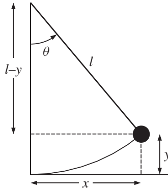
Figure 1.15 The geometry of the simple pendulum.
