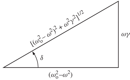
Figure 3.4 Geometrical construction for the phase angle \delta .
