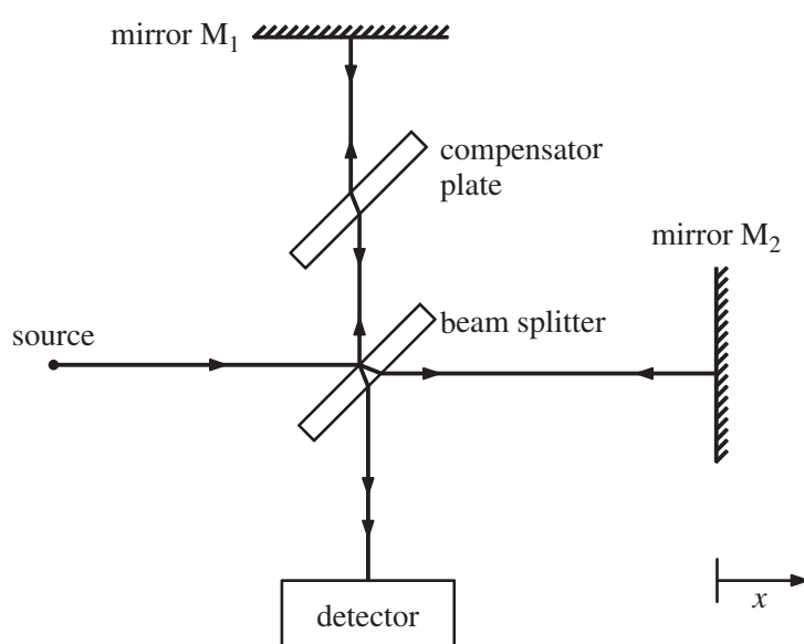
Figure 7.8 Schematic diagram of the Michelson spectral interferometer.
