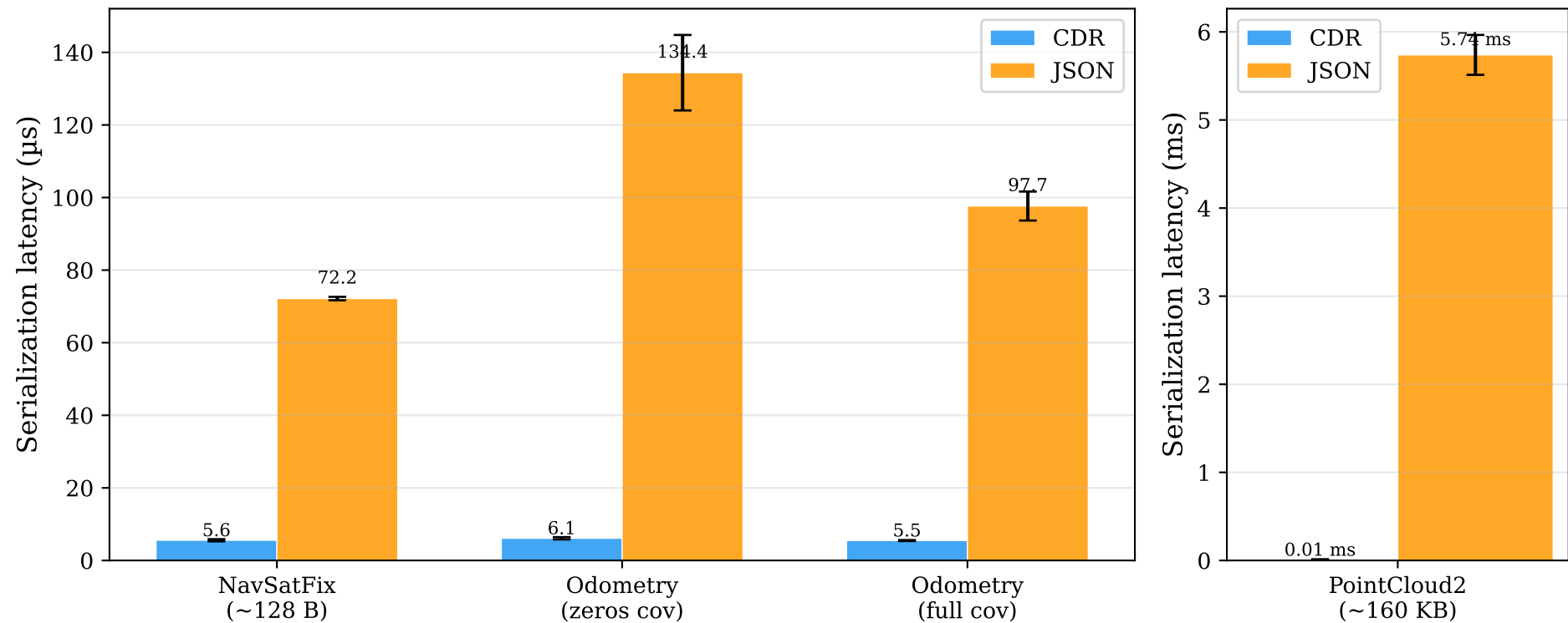
Average Serialization Latency — CDR vs JSON (10 Hz)
