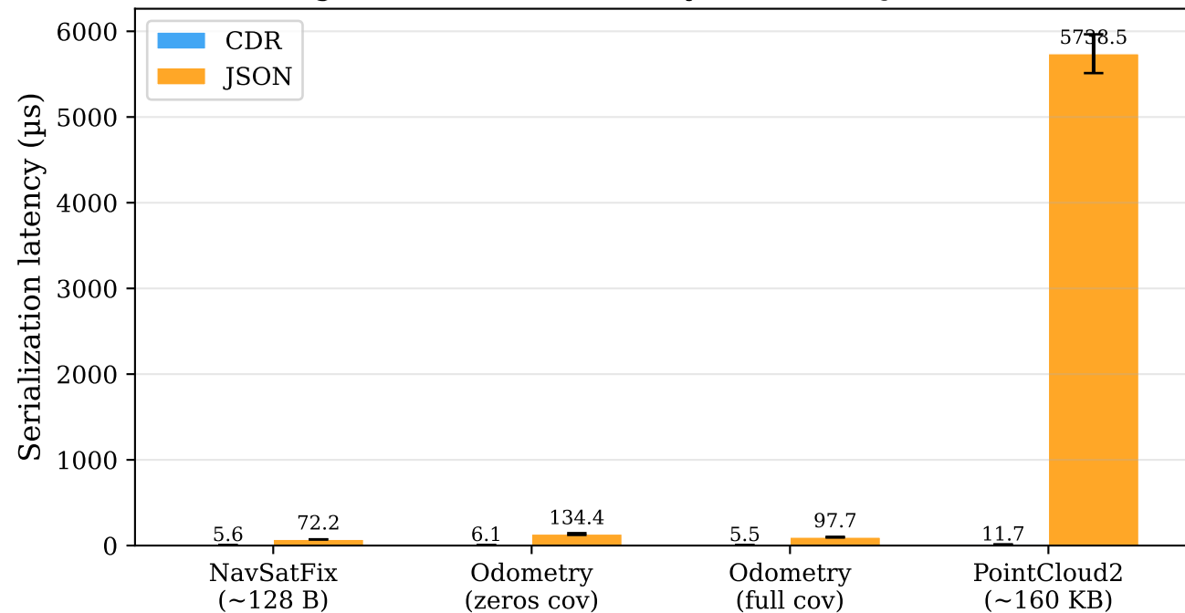
Average Serialization Latency — CDR vs JSON (10 Hz)
