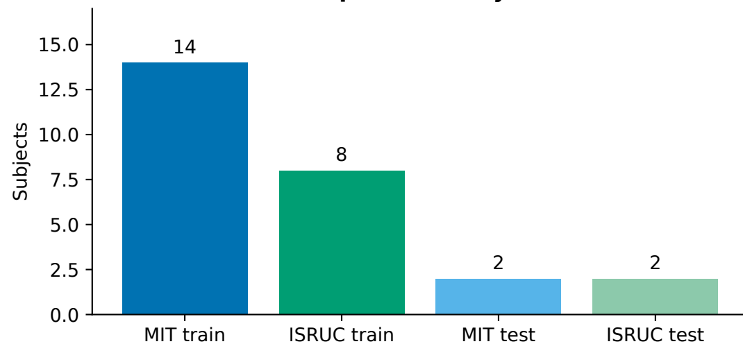
Independent subjects
