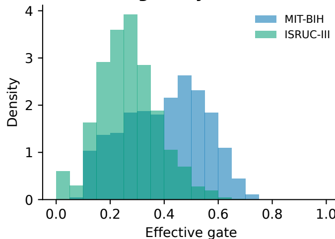
A5: gate by dataset
