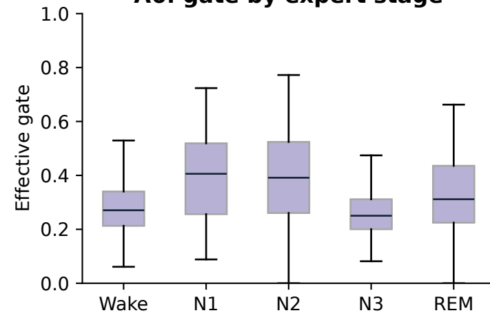
A6: gate by expert stage
