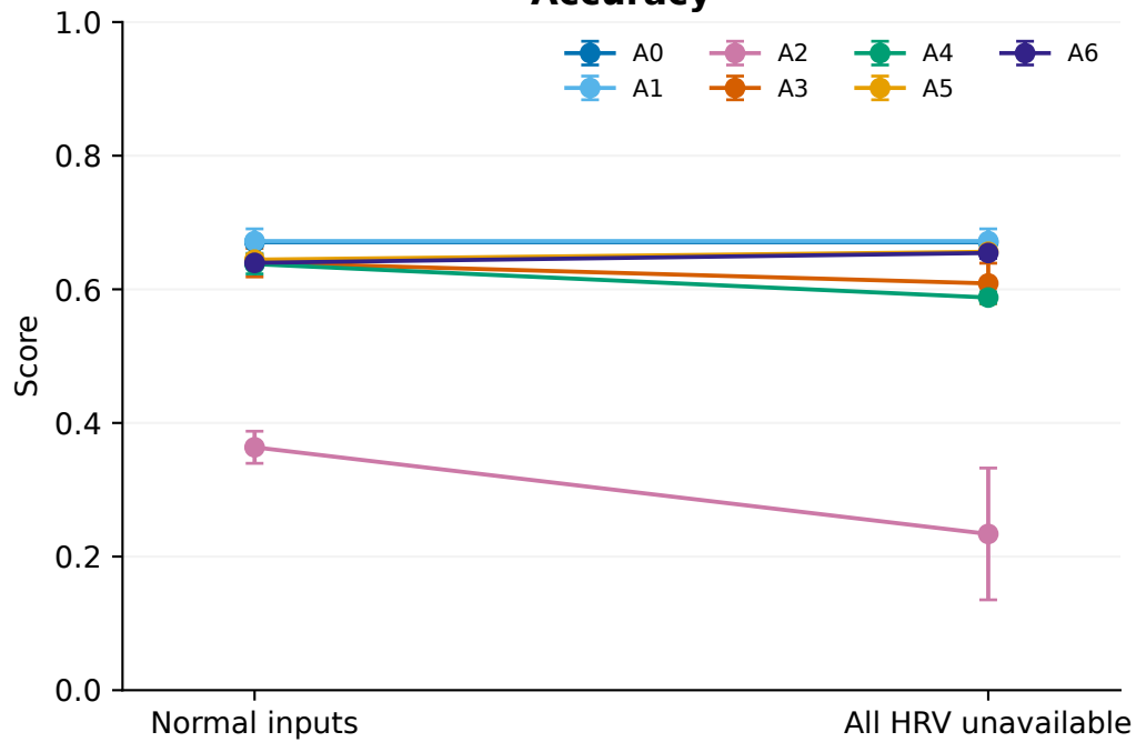
Accuracy
