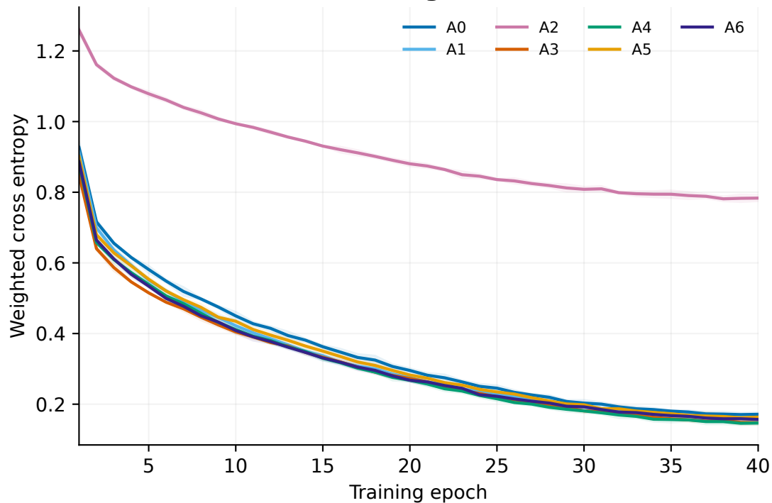
Training loss
