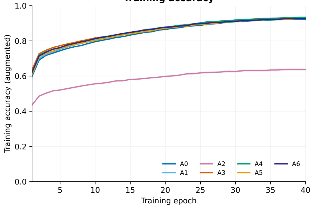
Training accuracy
