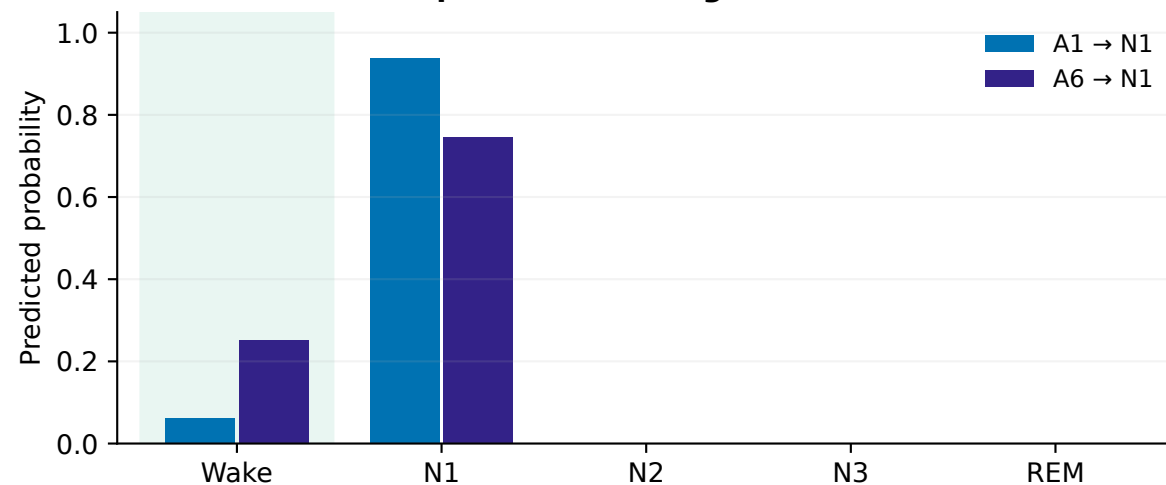
Both wrong · ISRUC-III-04 / epoch 26 Expert: Wake · A6 gate=0.333
