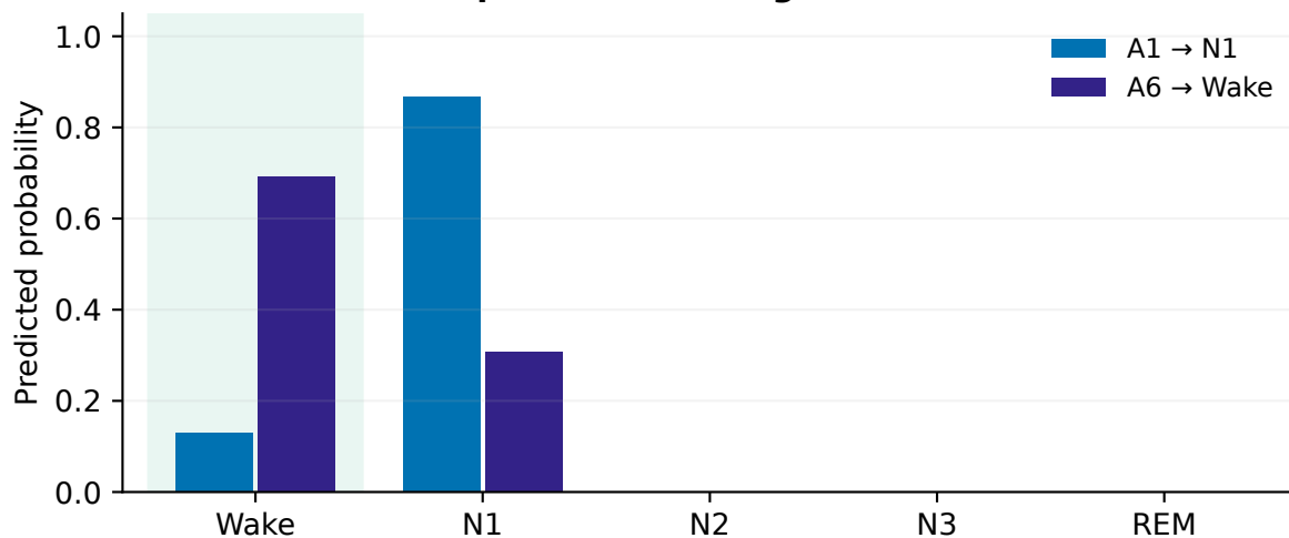
Only A6 correct · ISRUC-III-04 / epoch 27 Expert: Wake · A6 gate=0.218
