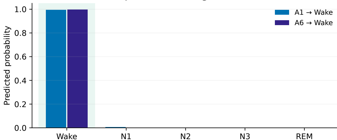
Both correct · ISRUC-III-04 / epoch 14 Expert: Wake · A6 gate=0.301
