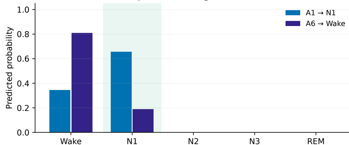
Only A1 correct · ISRUC-III-04 / epoch 29 Expert: N1 · A6 gate=0.198
