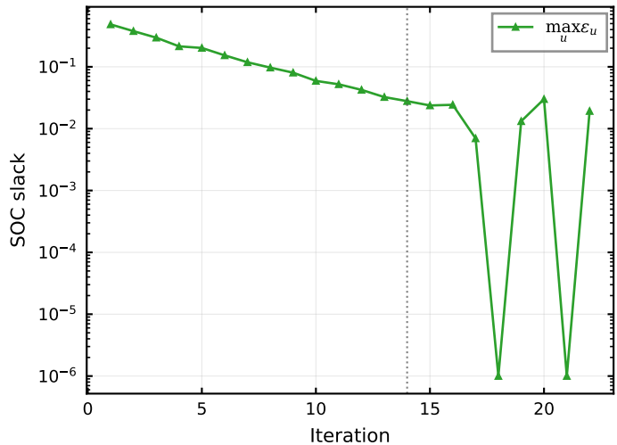
Example: ADMM convergence trajectory
