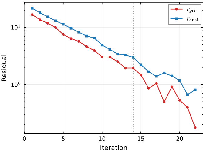
Example: ADMM convergence trajectory
