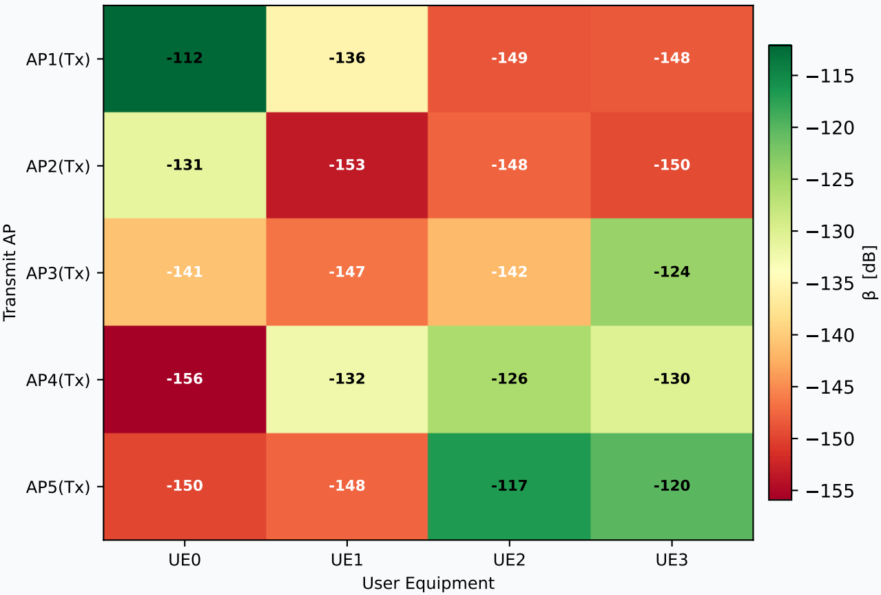
Large-Scale Fading \beta [dB]
