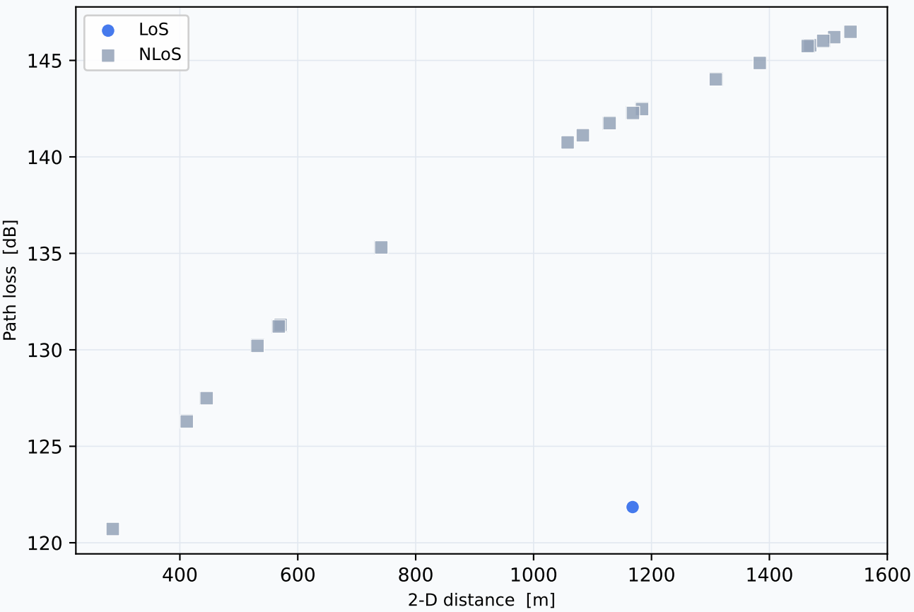
Path Loss vs. 2-D Distance
