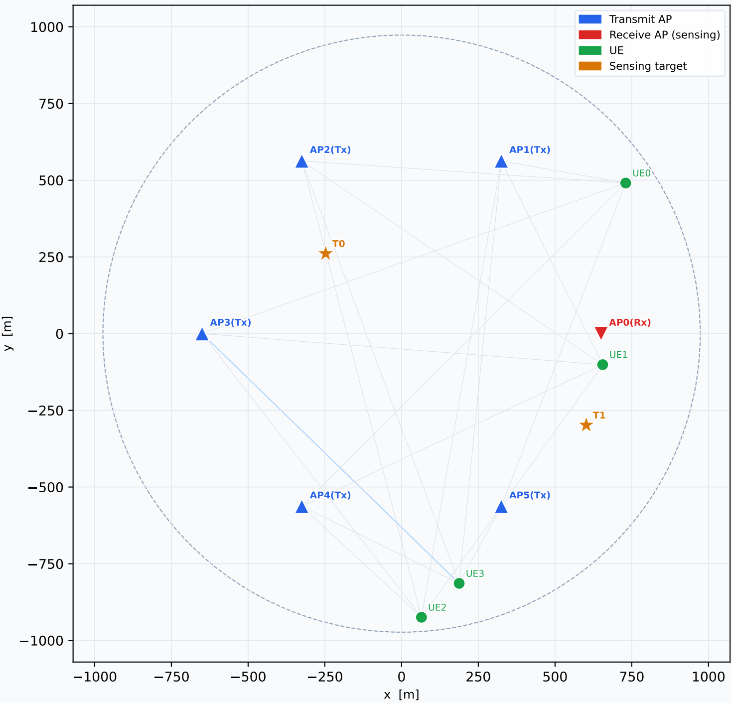
Network Topology (seed42_circle_6ap) 6 APs (Tx=5, Rx=1) | 4 UEs | 2 Targets
