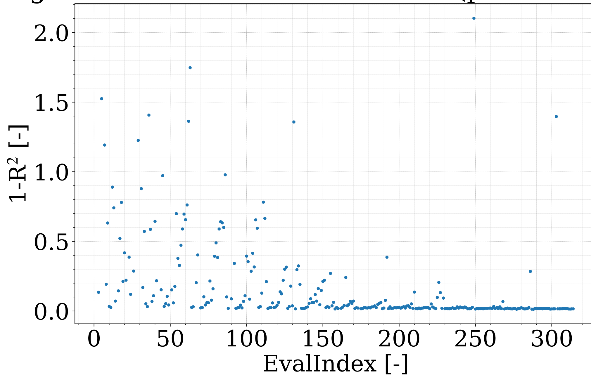
Convergence of evaluated individuals (penalized excluded)
