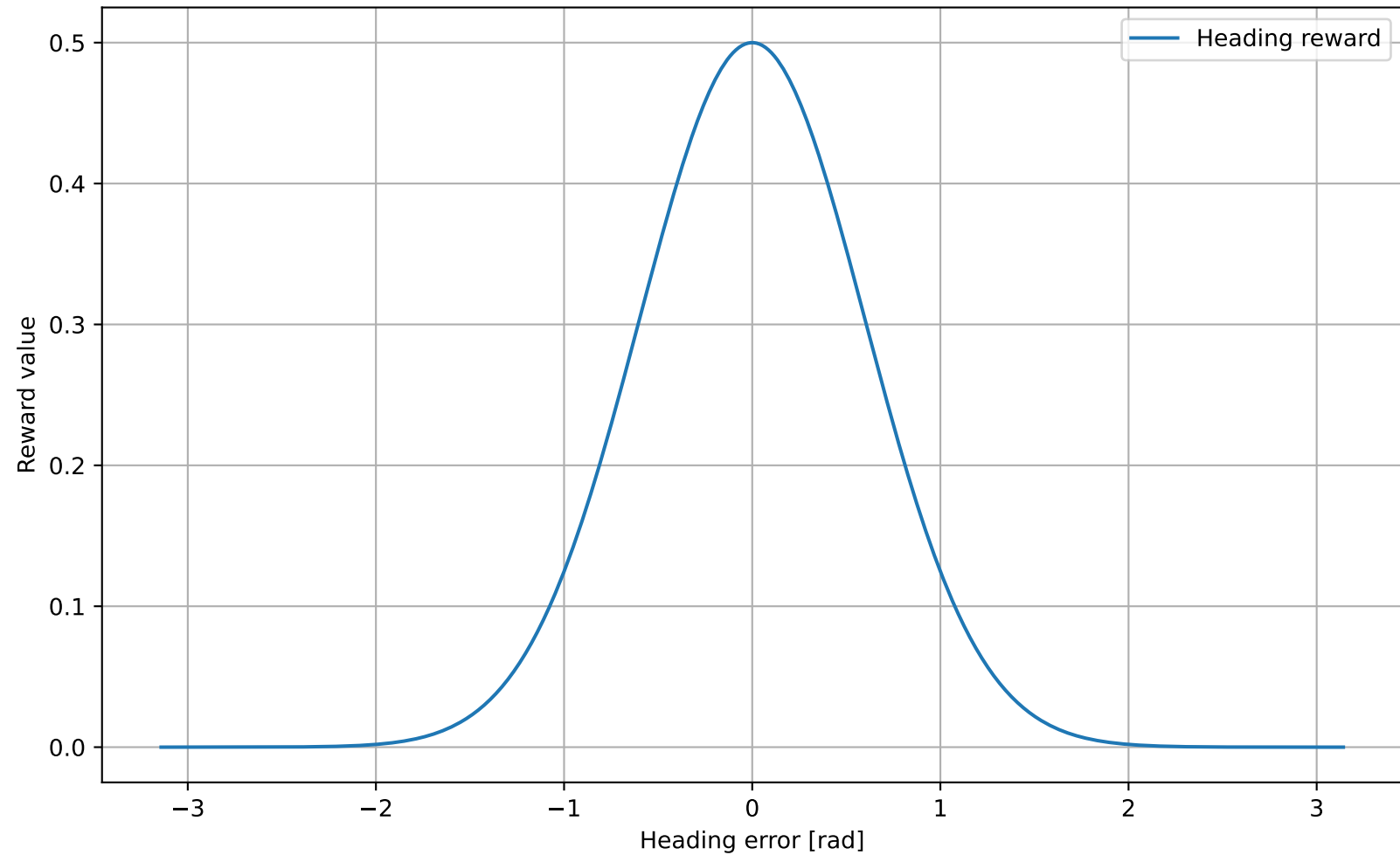
Heading reward
