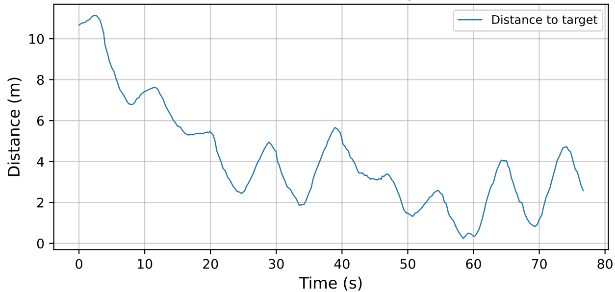
DRL distance to target
