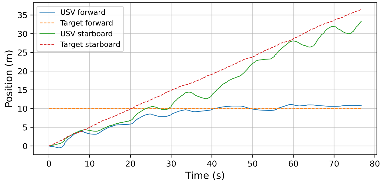
DRL position components
