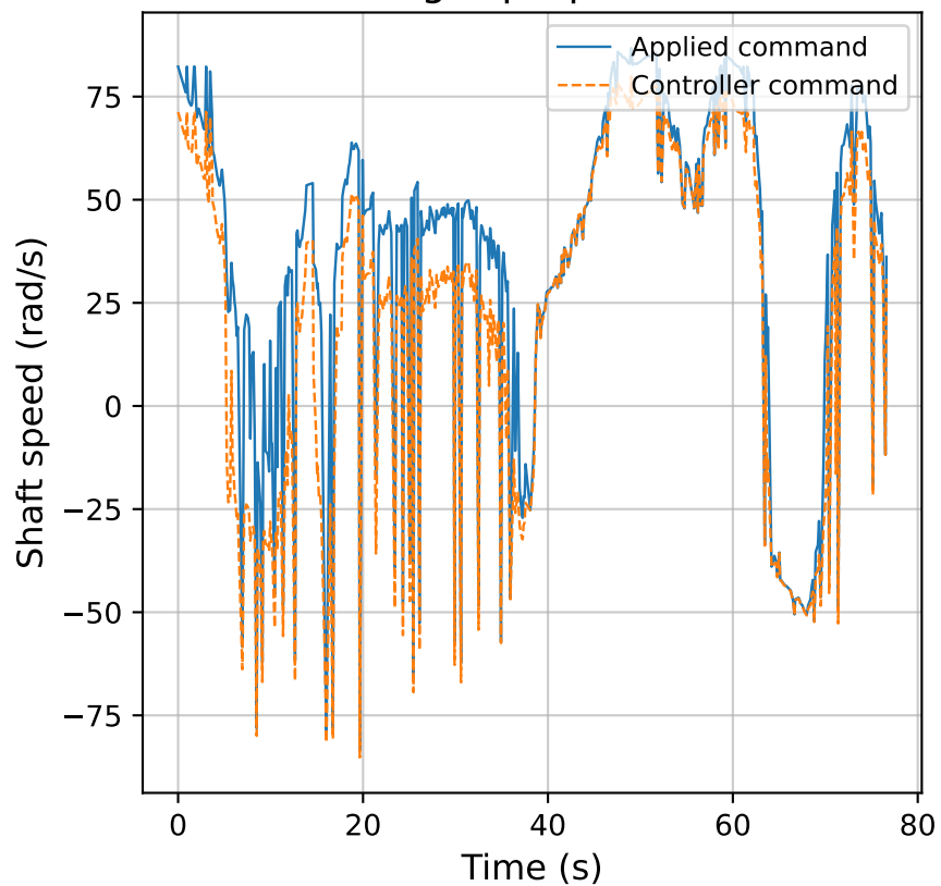
Right propeller
