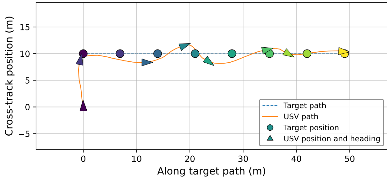
NMPC target tracking
