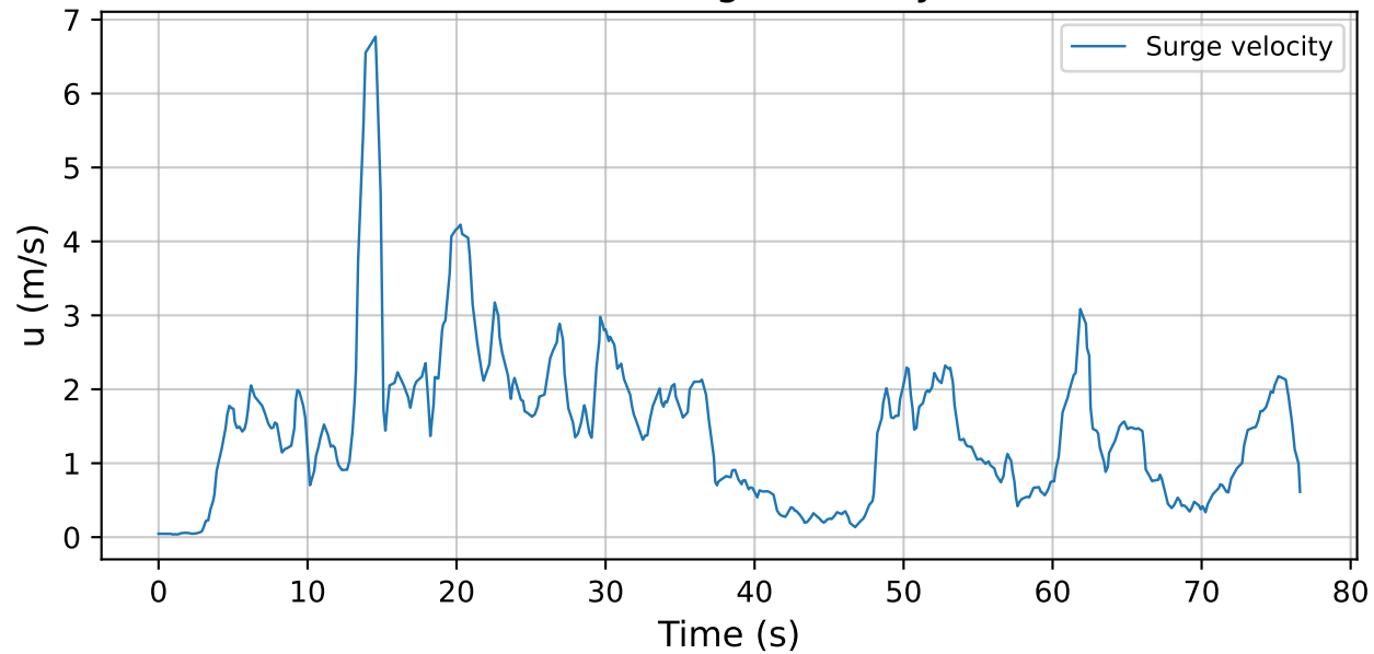
NMPC surge velocity
