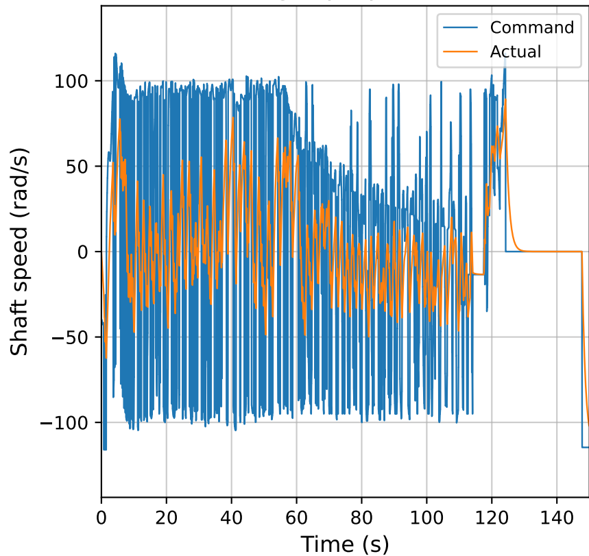
Right propeller
