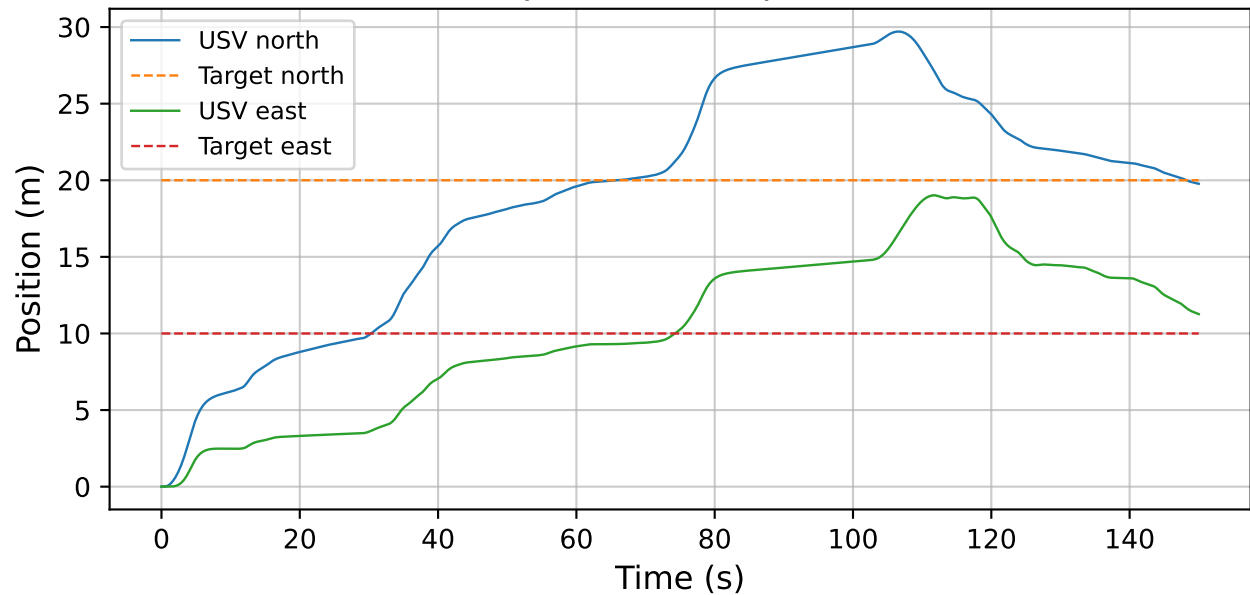
PID position components
