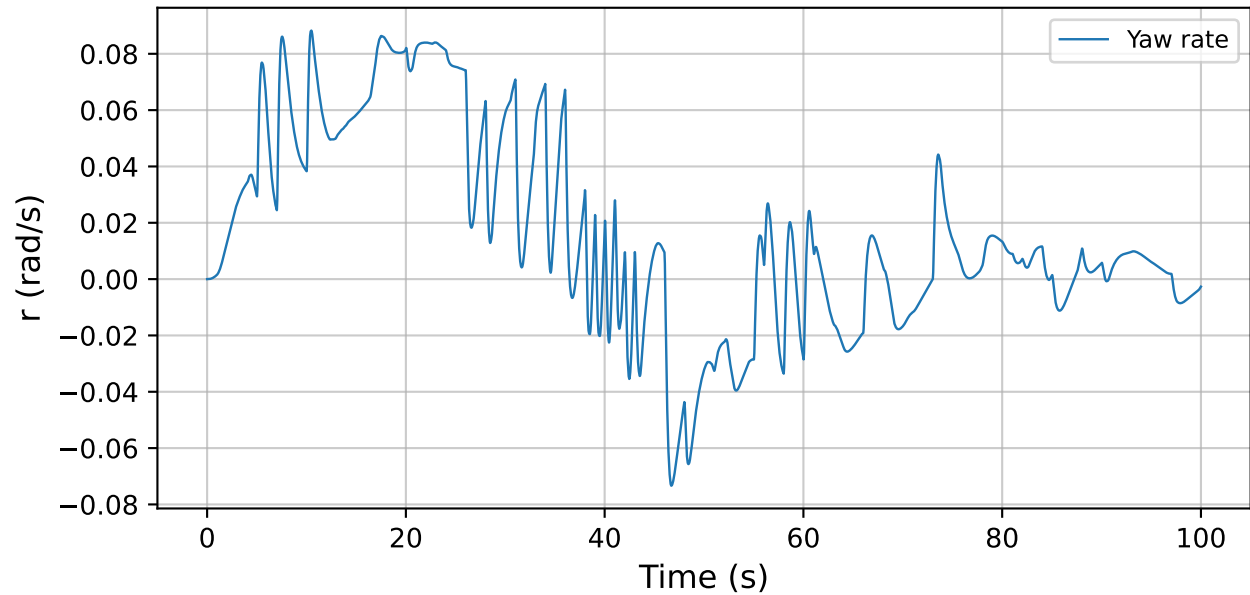
PID yaw rate
