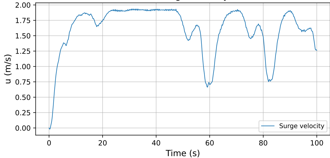
DRL surge velocity
