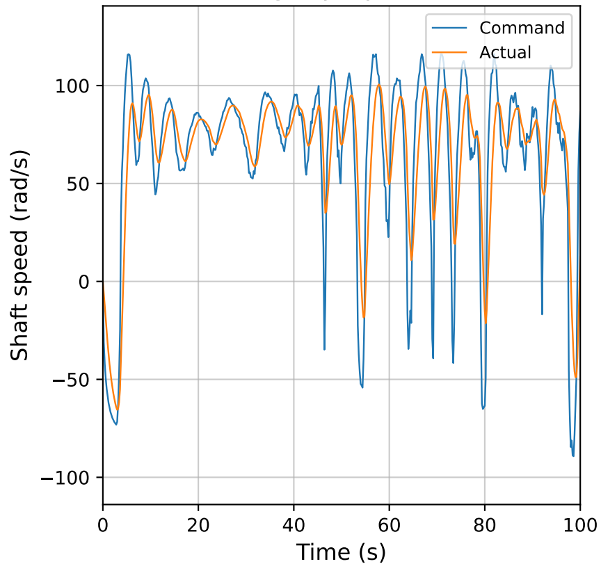
Right propeller
