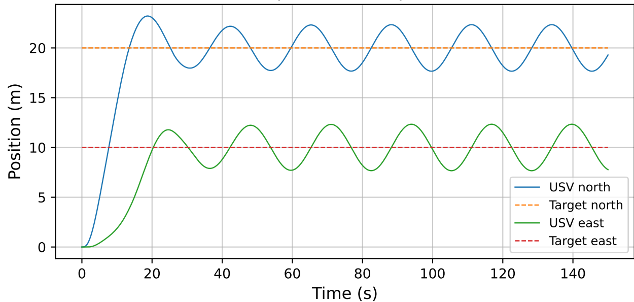
NMPC position components
