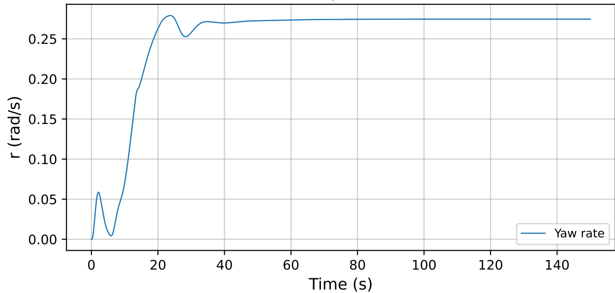
NMPC yaw rate
