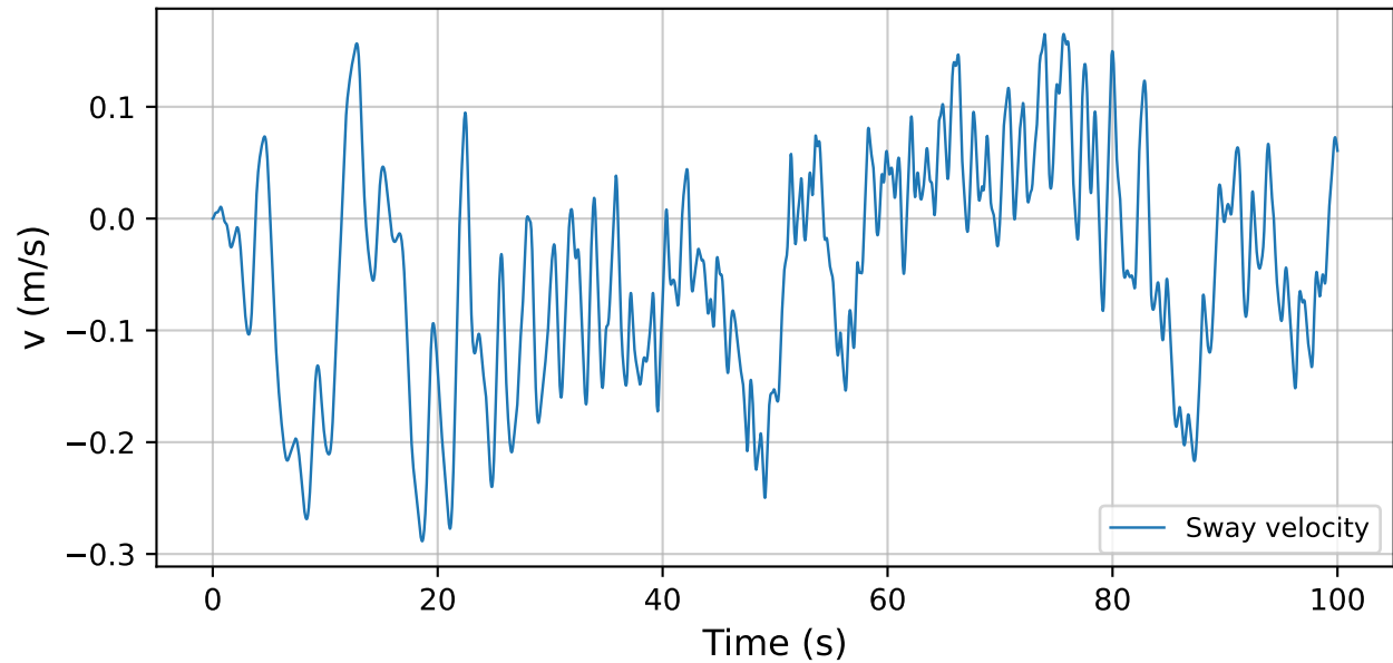
NMPC sway velocity
