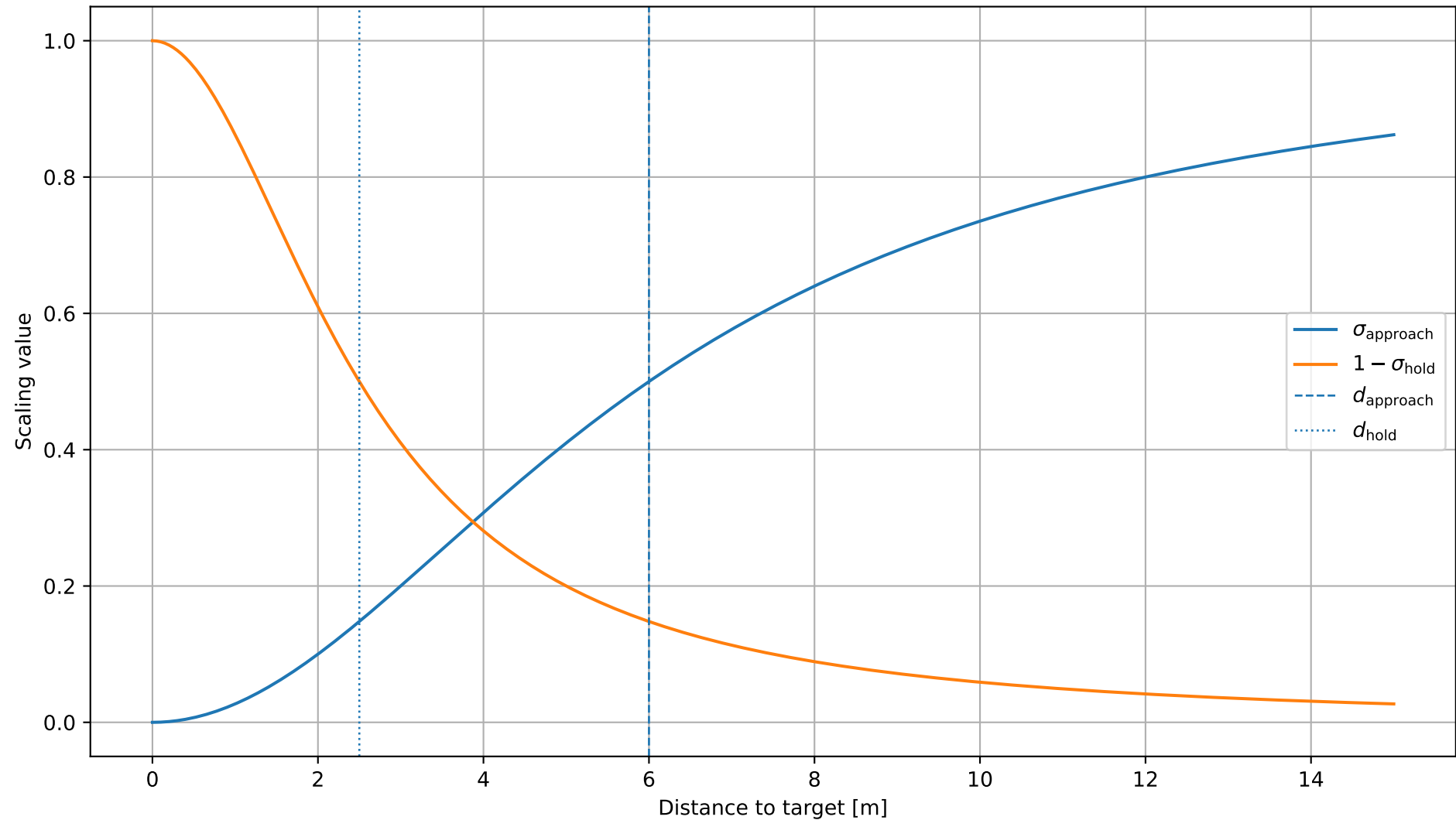
NMPC dynamic-positioning distance scaling
