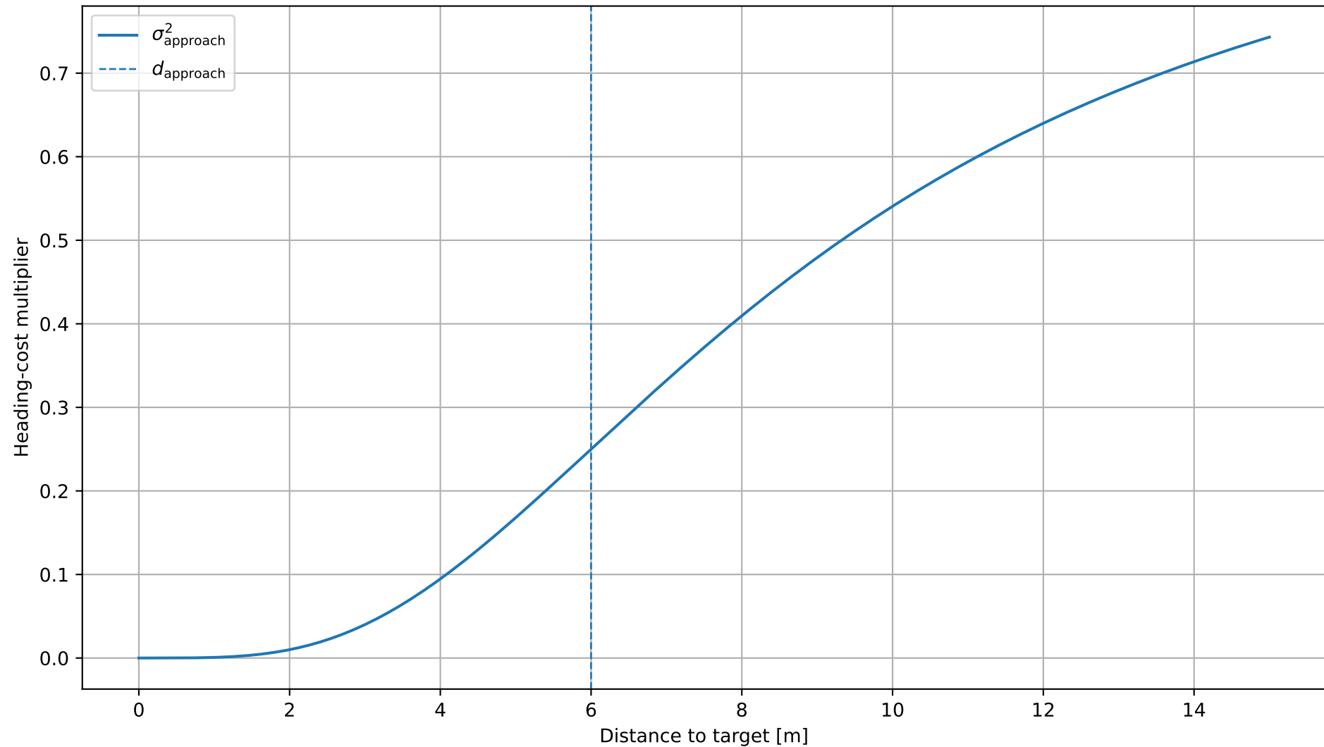
Heading-cost scaling for dynamic positioning
