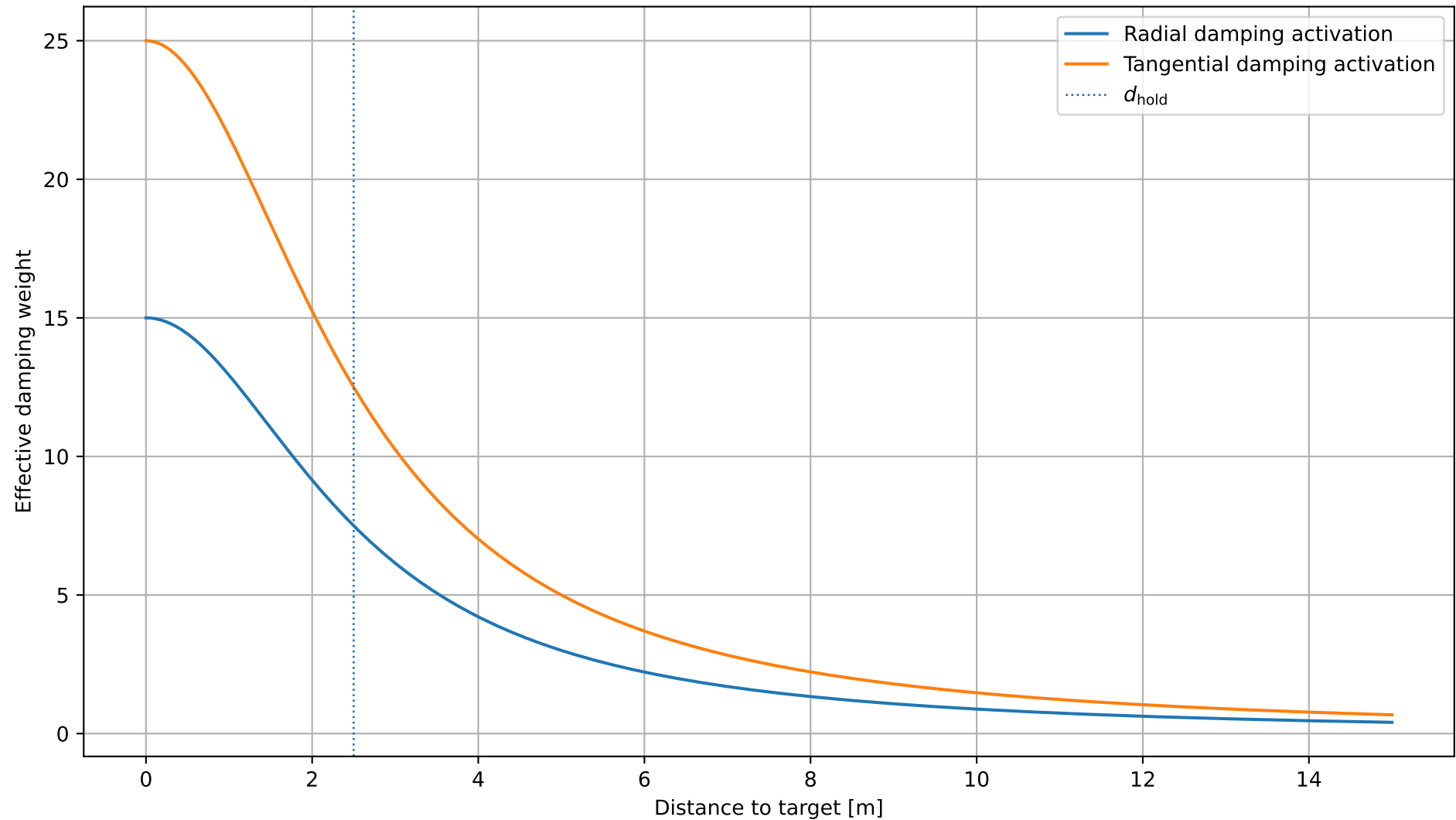
Velocity-damping activation for dynamic positioning
