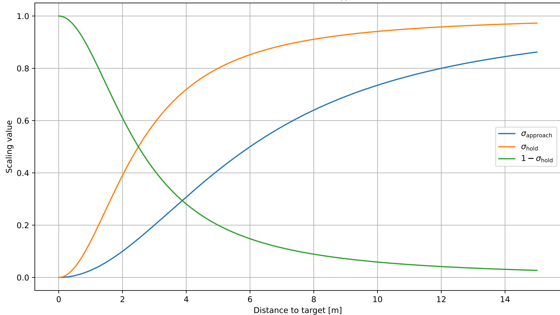
NMPC dynamic-positioning distance scaling ( d_{\text{approach}} = 6.0 m, d_{\text{hold}} = 2.5 m)
