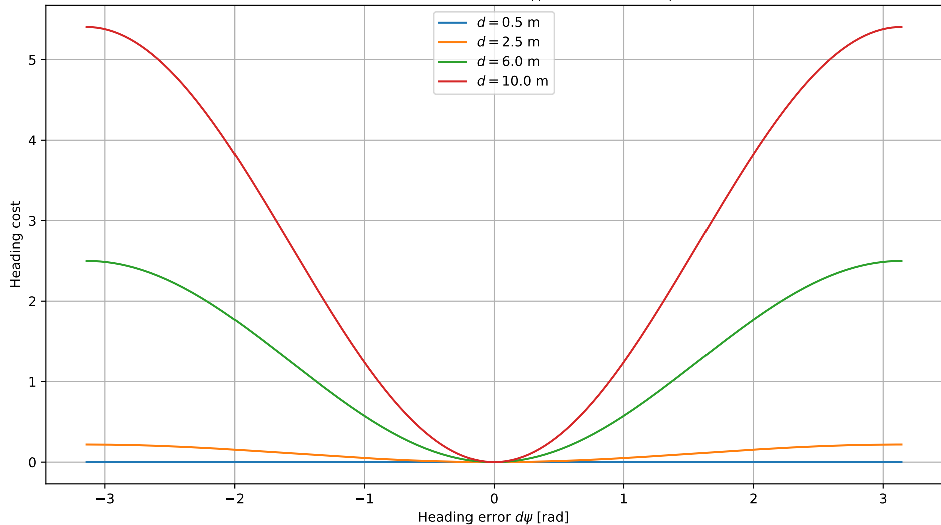
Heading cost vs heading error ( d_{\text{approach}} = 6.0 m, w_{\psi} = 5.0 )
