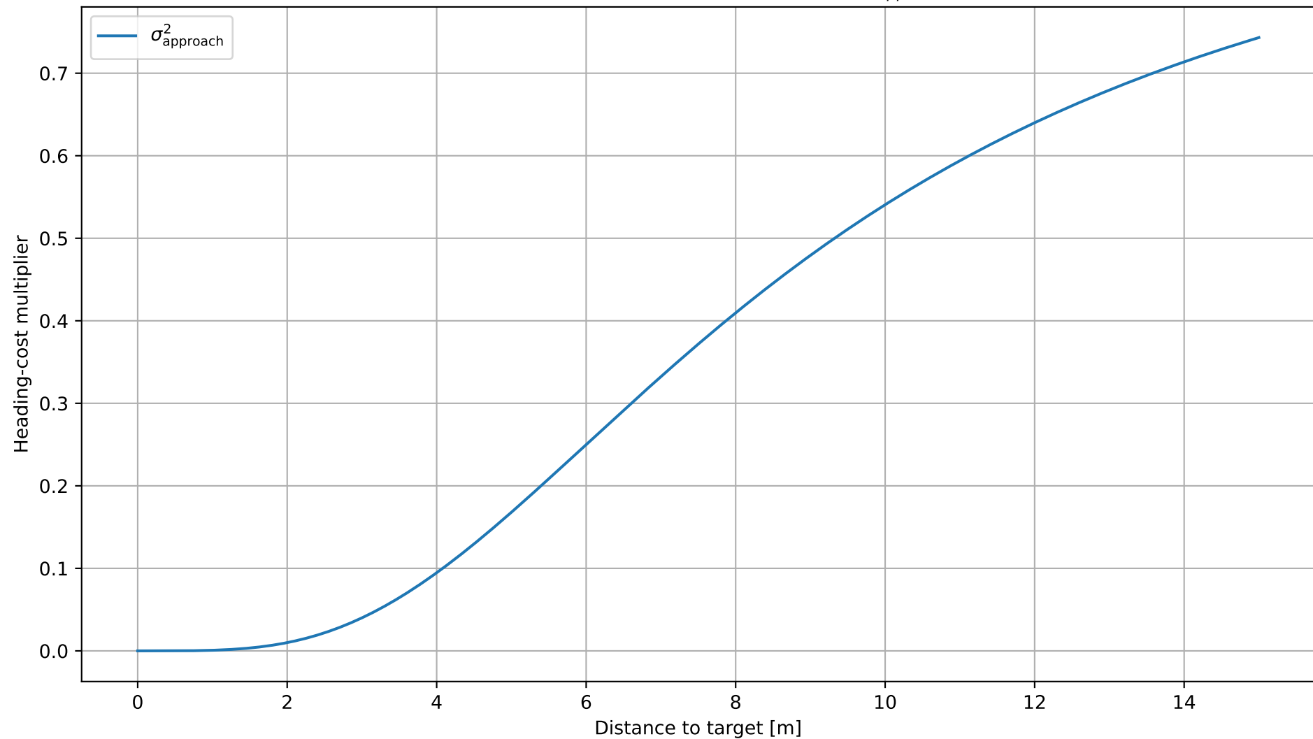
Heading-cost scaling for dynamic positioning ( d_{\text{approach}} = 6.0 m)
