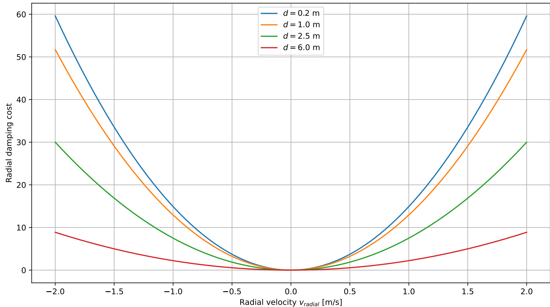
Radial damping cost vs radial velocity ( d_{hold} = 2.5 m, w_r = 15.0 )
