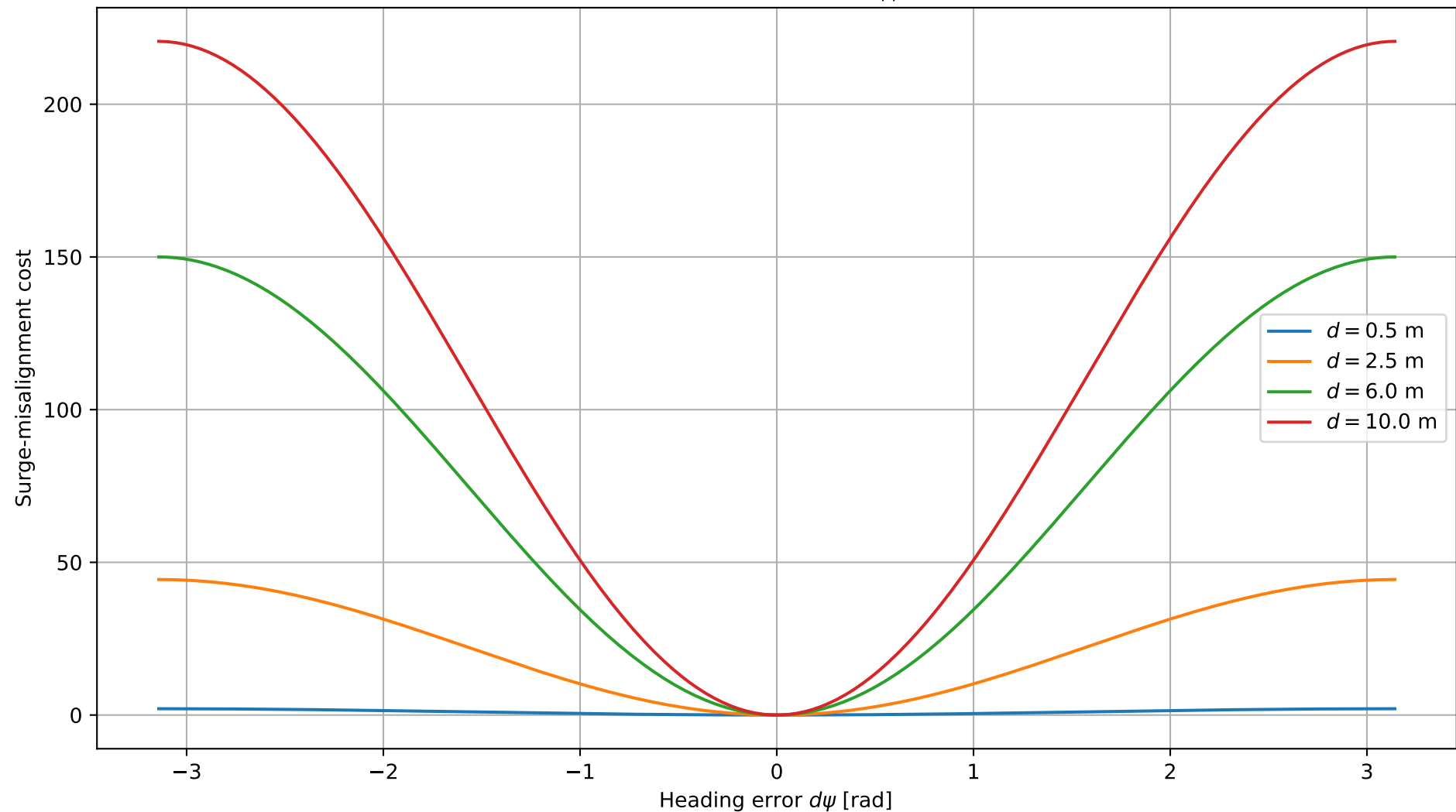
Surge-misalignment cost vs heading error ( d_{\text{approach}} = 6.0 m, \tau_\chi = 100.0 N)
