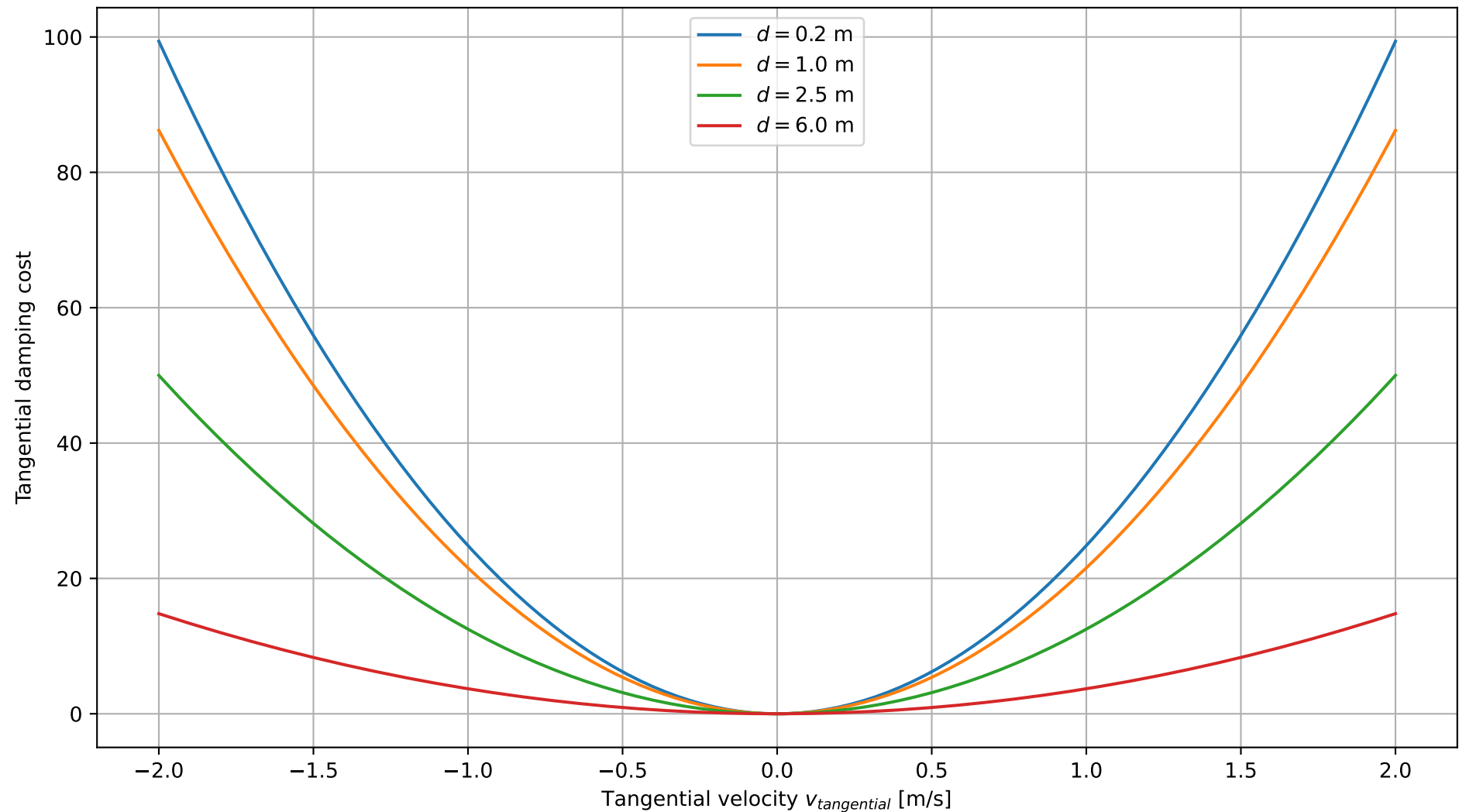
Tangential damping cost vs tangential velocity ( d_{hold} = 2.5 m, w_t = 25.0 )
