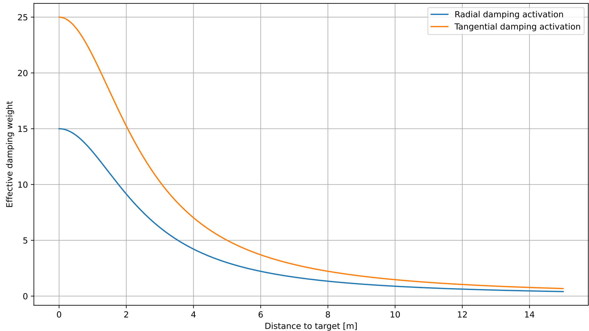
Velocity-damping activation for dynamic positioning ( d_{hold} = 2.5 m, w_r = 15.0 , w_t = 25.0 )
