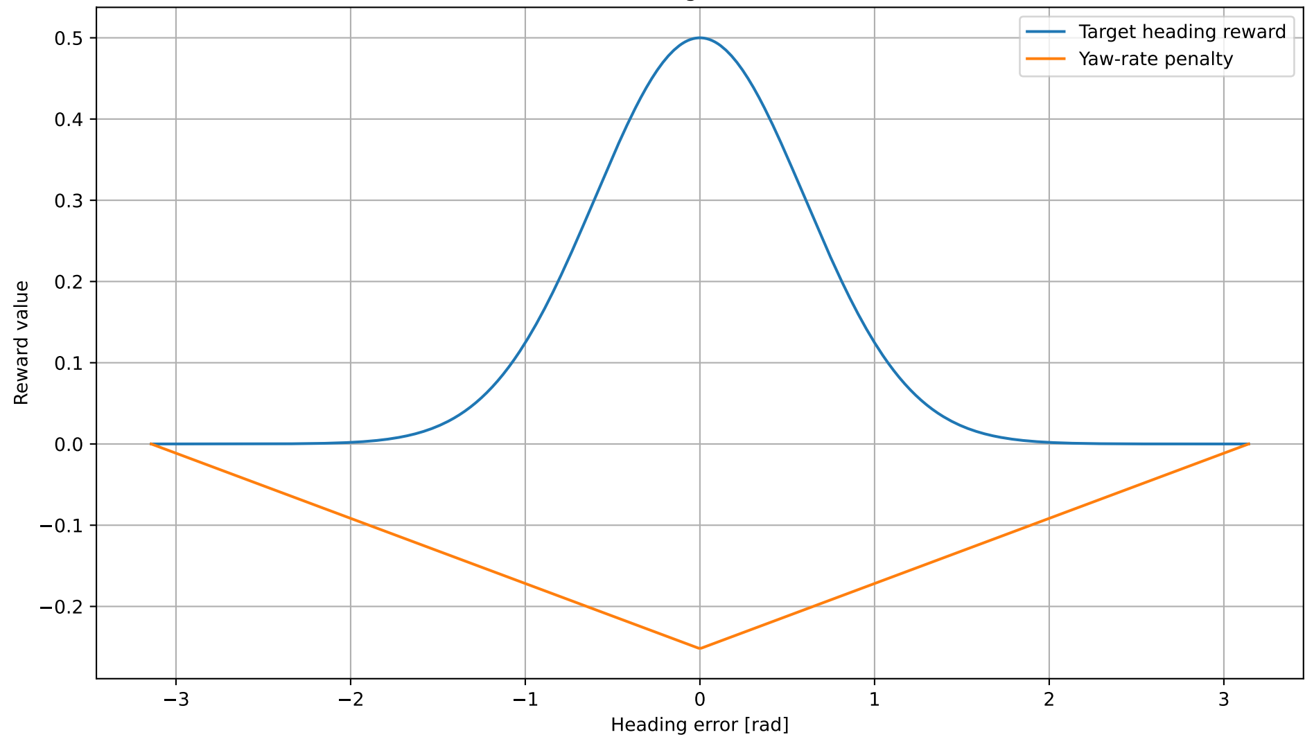
Heading rewards
