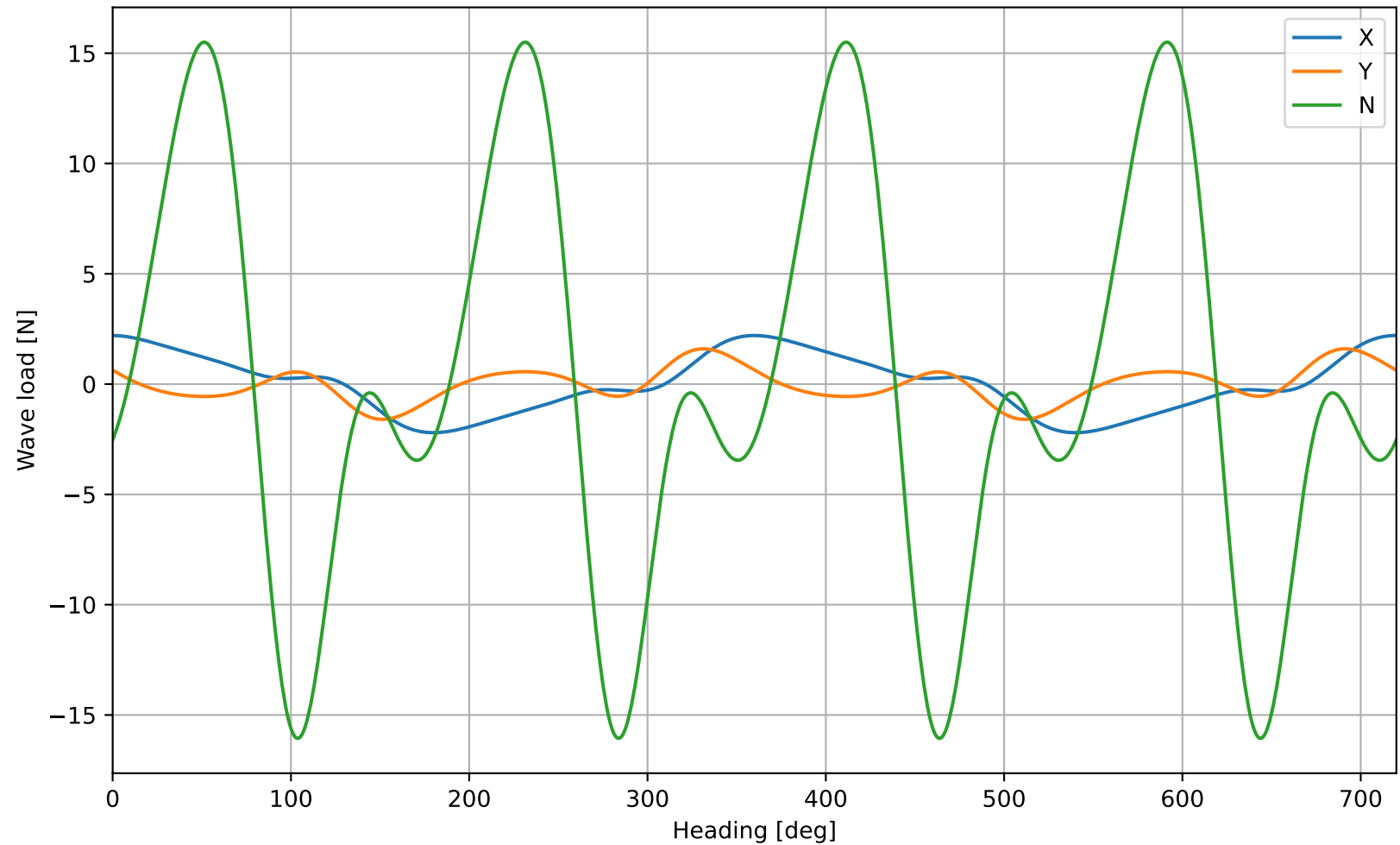
Wave loads vs heading
