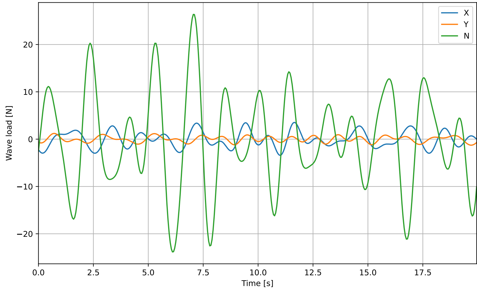
Wave loads vs time
