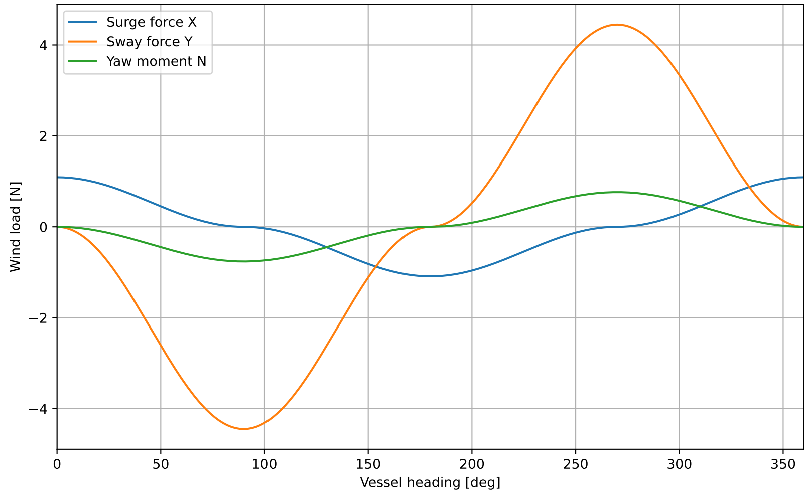
Wind loads vs heading
