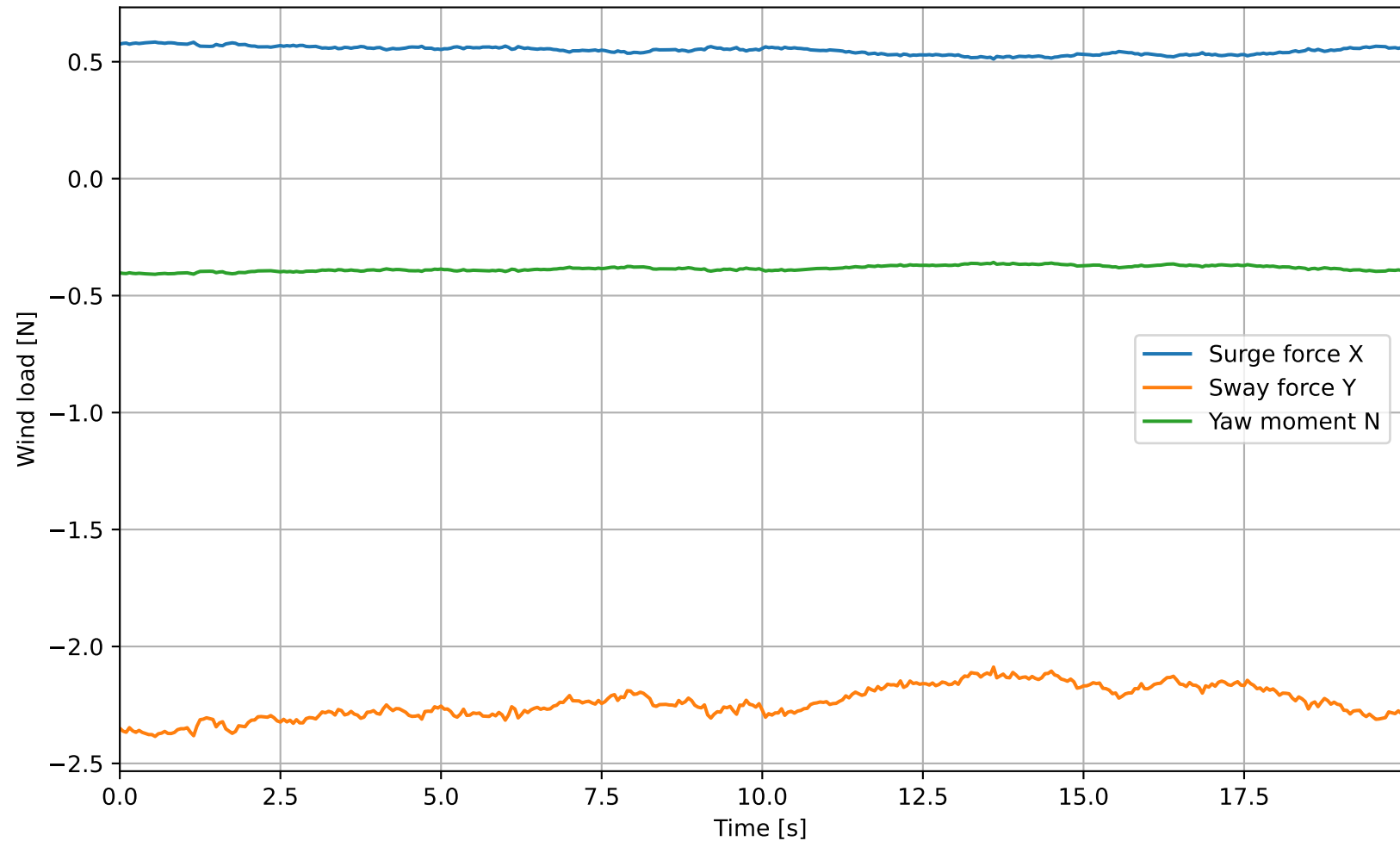
Wind loads vs time (45° heading)
