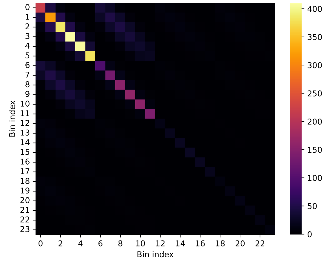
Cluster covariance (SN + SSC)
