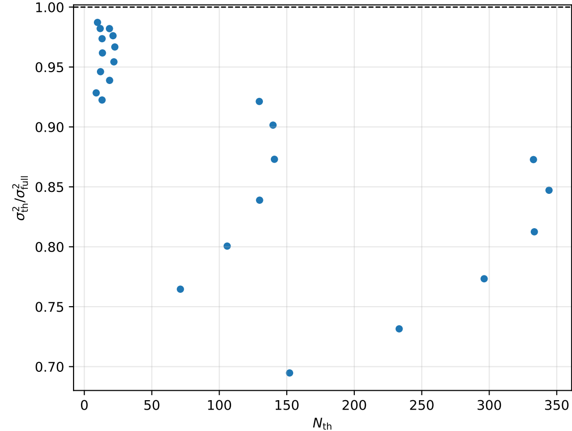
Shot noise contribution
