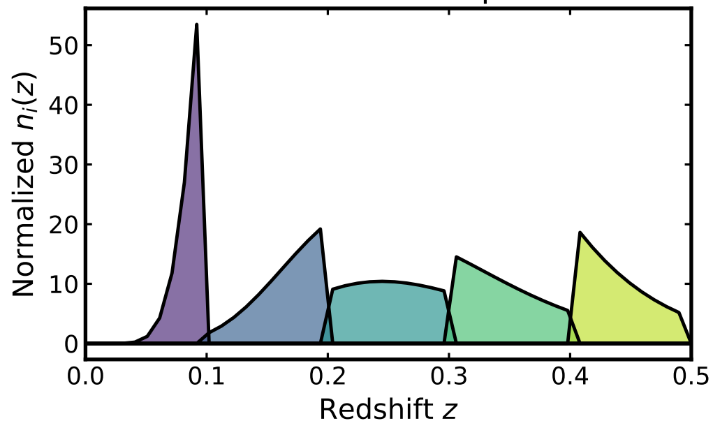
4MOST-CRS BG: five spec- z bins
