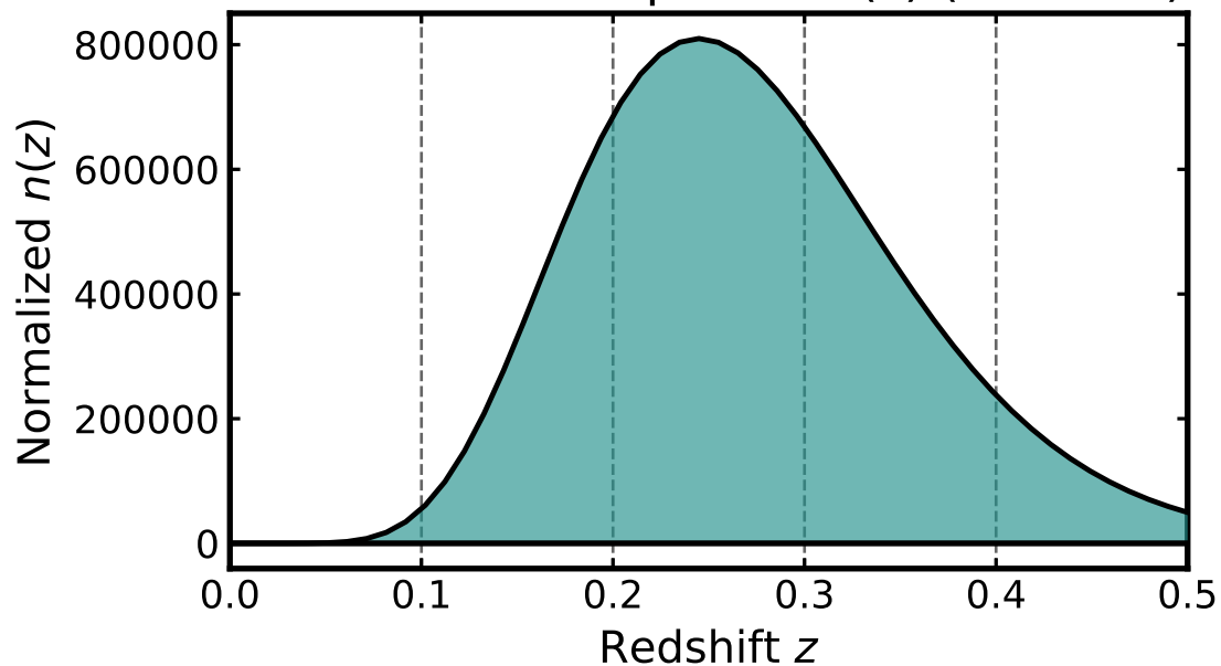
4MOST-CRS BG: parent n(z) (Smail fit)
